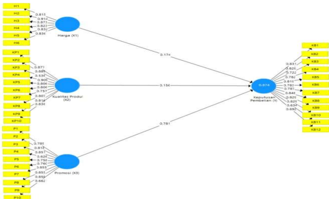
Gambar 2. Outlier Model
